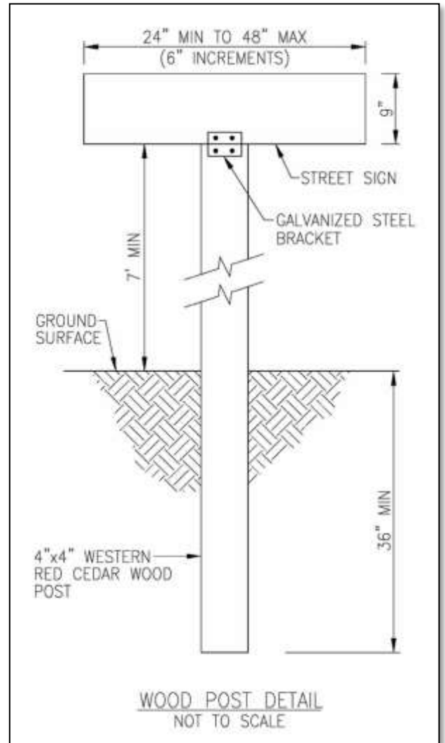
Exhibit B – Wood Post Detail
