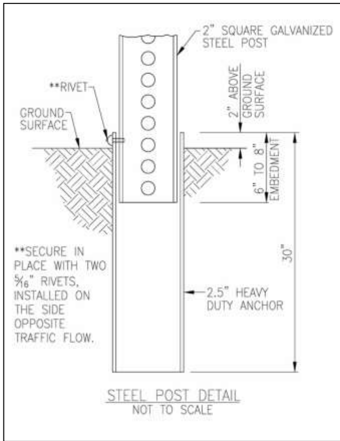
Exhibit A – Steel Post Detail
